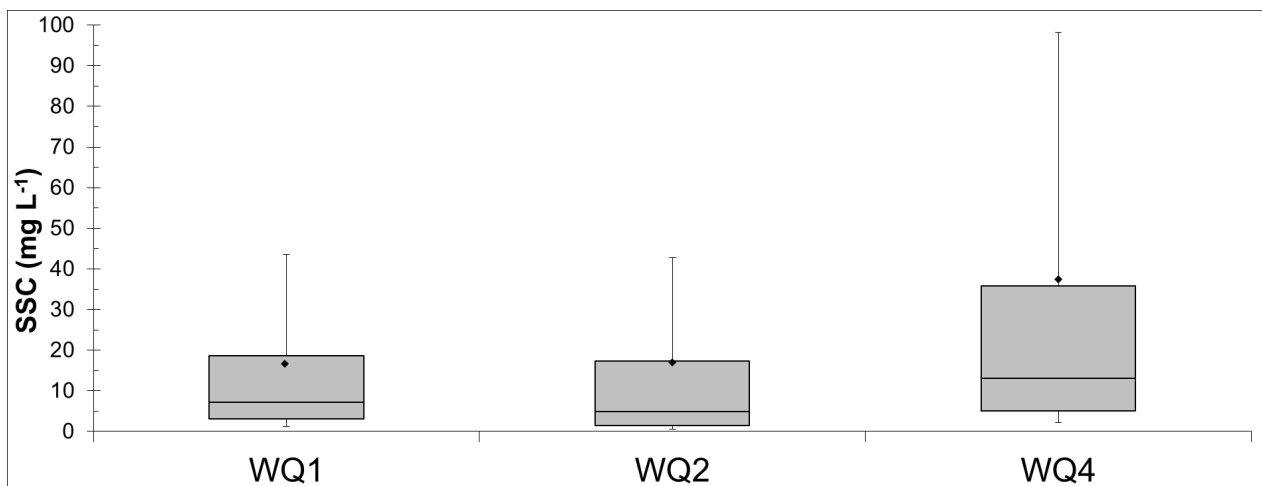
Figure 3.14 Box plot of SSC ( \text{mg L}^{-1} ) from July 2020 to July 2021. The lower whisker, lower edge of the box, central line, upper edge of the box and upper whisker represent the 10 th , 25 th , 50 th , 75 th and 90 th percentiles, respectively. The diamond represents the mean value.
