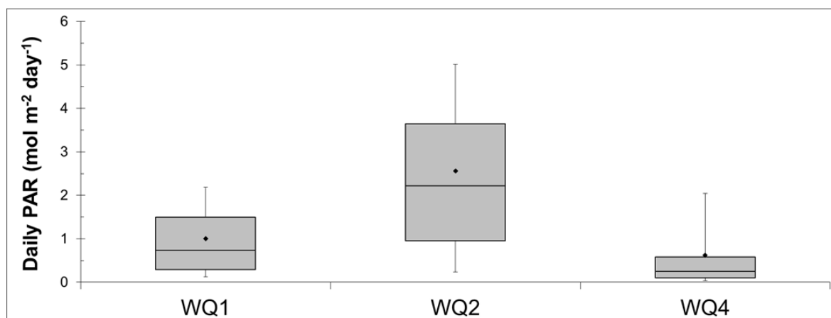
Figure 3.17 Box plot of daily PAR ( mol\ m^{-2}\ day^{-1} ) from July 2020 to July 2021. The lower whisker, lower edge of the box, central line, upper edge of the box and upper whisker represent the 10 th , 25 th , 50 th , 75 th and 90 th percentiles, respectively. The diamond represents the mean value.
