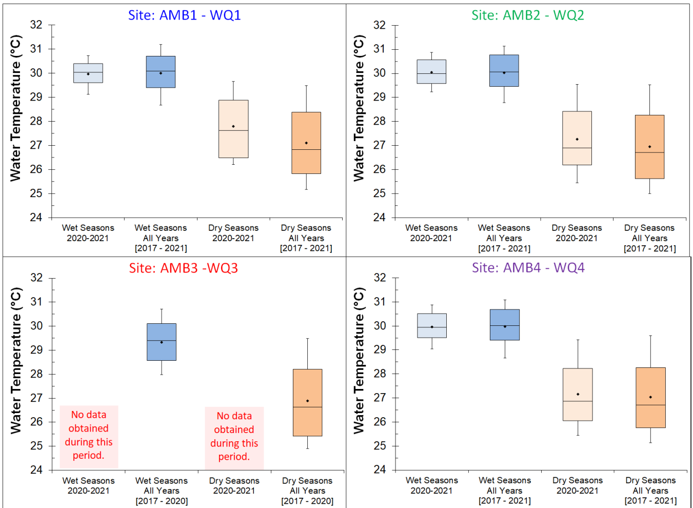
Figure 3.25 Water Temperature box plots for WQ1-WQ4. Blue boxes represent data that is within the Wet Season period (1 November-31 March) while orange boxes represent data that is within the Dry Season period (1 April-31 October). In addition, a comparison is made between this year’s observational period (2020 July -2021 July) and all available historical data (collectively, 2017-2021).
