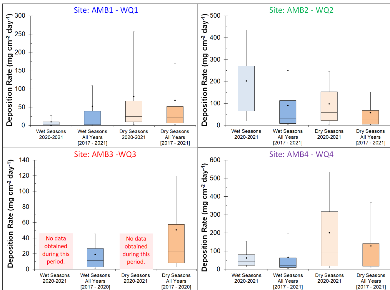
Figure 3.23 Deposition box plots for WQ1-WQ4. Blue boxes represent data that is within the Wet Season period (1 November-31 March) while orange boxes represent data that is within the Dry Season period (1 April-31 October). In addition, a comparison is made between this year’s observational period (2020 July -2021 July) and all available historical data (collectively, 2017-2021).
