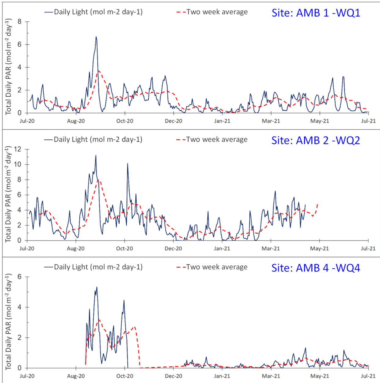
Figure 3.18 Time series of total daily PAR (mol m -2 day -1 ) from July 2020 to July 2021. Daily mean PAR is plotted in blue and a 2-week moving average of daily mean PAR is plotted in red.
