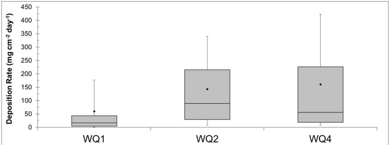
Figure 3.15 Box plot of deposition rates ( \text{mg cm}^{-2} \text{day}^{-1} ) from July 2020 to July 2021. The lower whisker, lower edge of the box, central line, upper edge of the box and upper whisker represent the 10 th , 25 th , 50 th , 75 th and 90 th percentiles, respectively. The diamond represents the mean value.
