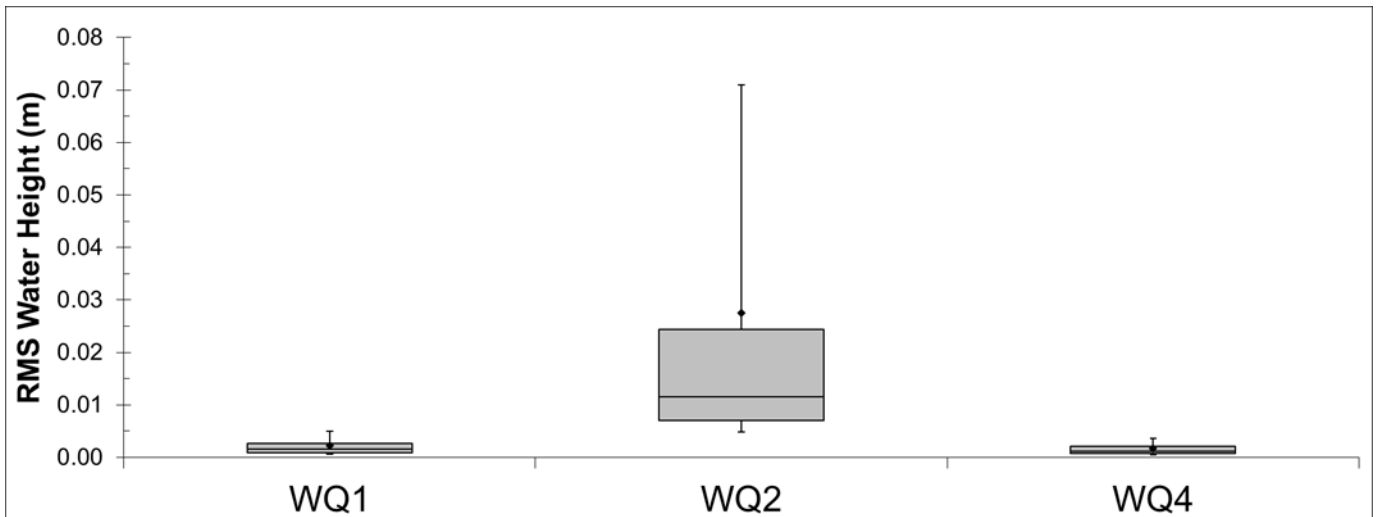
Figure 3.13 Box plot of root mean square (RMS) of water height (m) at the three sites for the monitoring period from July 2020 to July 2021. The lower whisker, lower edge of the box, central line, upper edge of the box and upper whisker represent the 10 th , 25 th , 50 th , 75 th and 90 th percentiles, respectively. The diamond represents the mean values.
