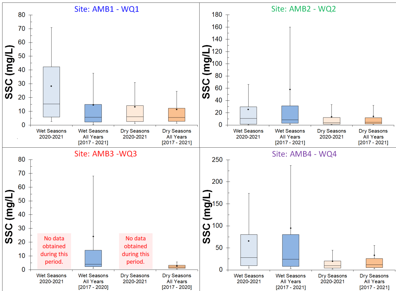
Figure 3.22 SSC box plots for WQ1-WQ4. Blue boxes represent data that is within the Wet Season period (1 November-31 March) while orange boxes represent data that is within the Dry Season period (1 April-31 October). In addition, a comparison is made between this year’s observational period (2020 July -2021 July) and all available historical data (collectively, 2017-2021).
