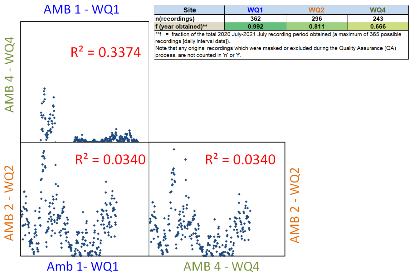
Figure 3.20 Scatterplots of PAR between sites indicating the strength of the relationships between patterns of daily PAR for July 2020 to July 2021. R^2 values are presented for each comparison.
