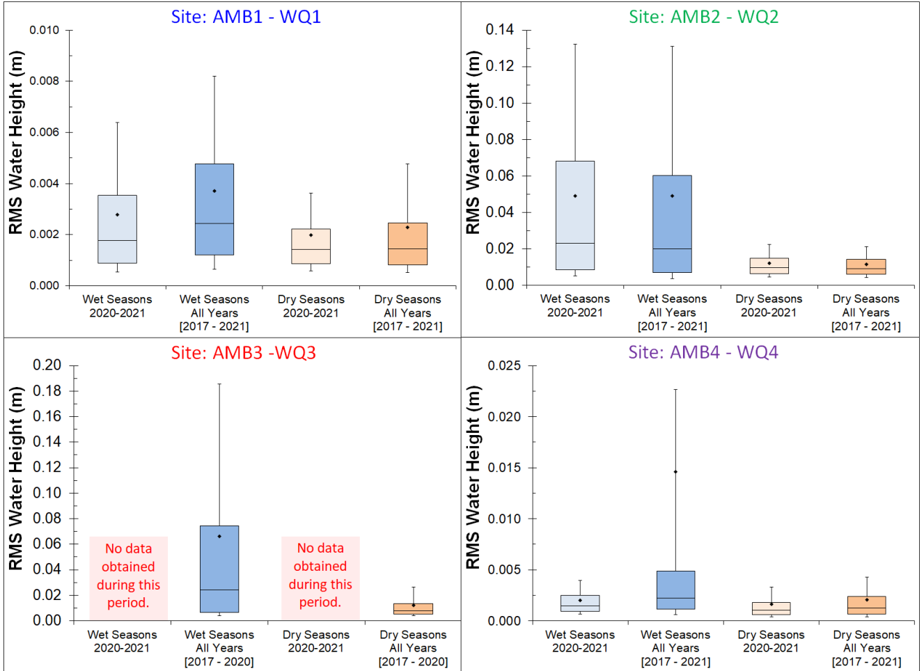
Figure 3.21 RMS box plots for WQ1-WQ4. Blue boxes represent data that is within the Wet Season period (1 November-31 March) while orange boxes represent data that is within the Dry Season period (1 April-31 October). In addition, a comparison is made between this year’s observational period (2020 July -2021 July) and all available historical data (collectively, 2017-2021).
