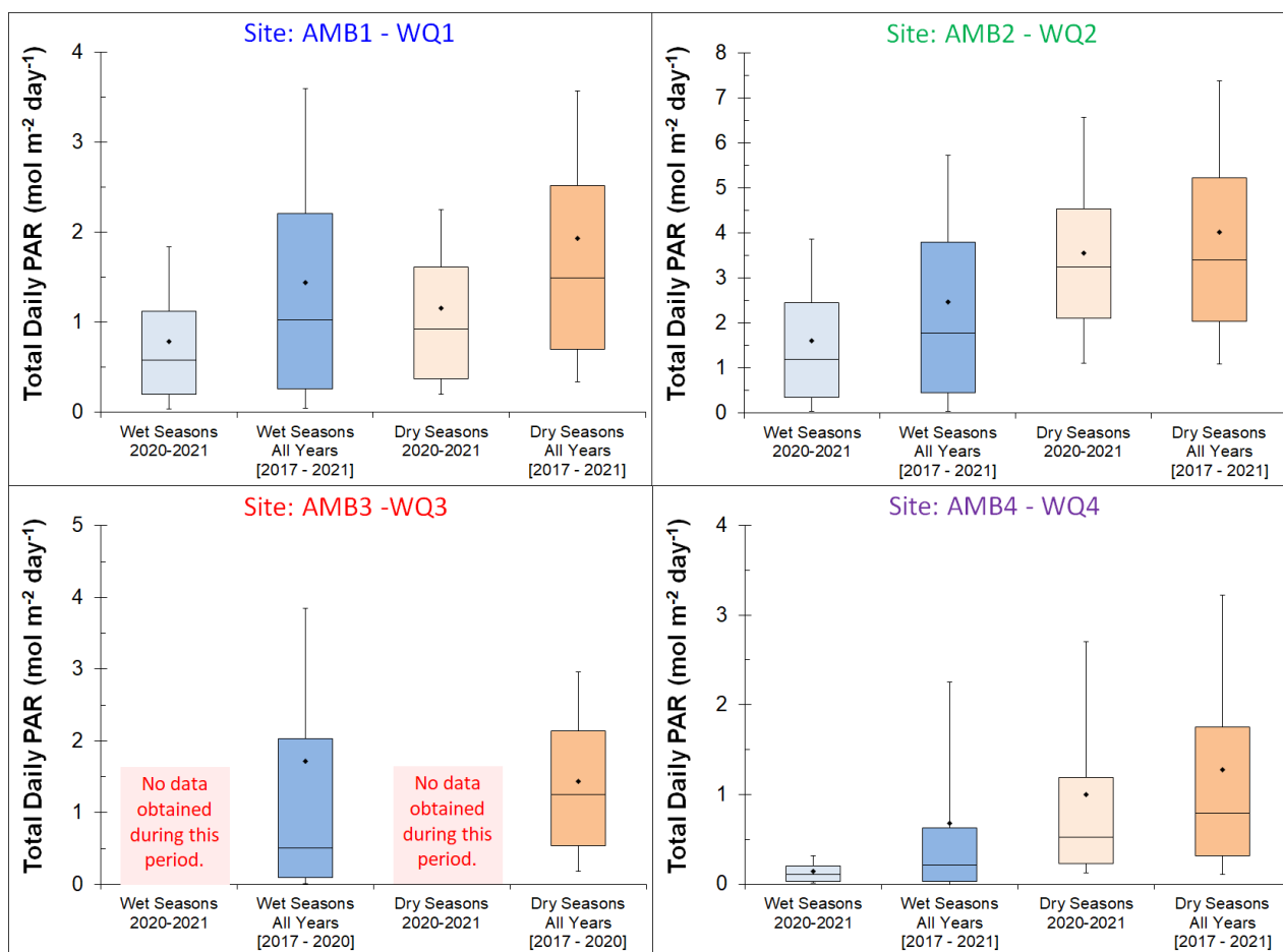
Figure 3.24 Total Daily PAR box plots for WQ1-WQ4. Blue boxes represent data that is within the Wet Season period (1 November-31 March) while orange boxes represent data that is within the Dry Season period (1 April-31 October). In addition, a comparison is made between this year’s observational period (2020 July -2021 July) and all available historical data (collectively, 2017-2021).
