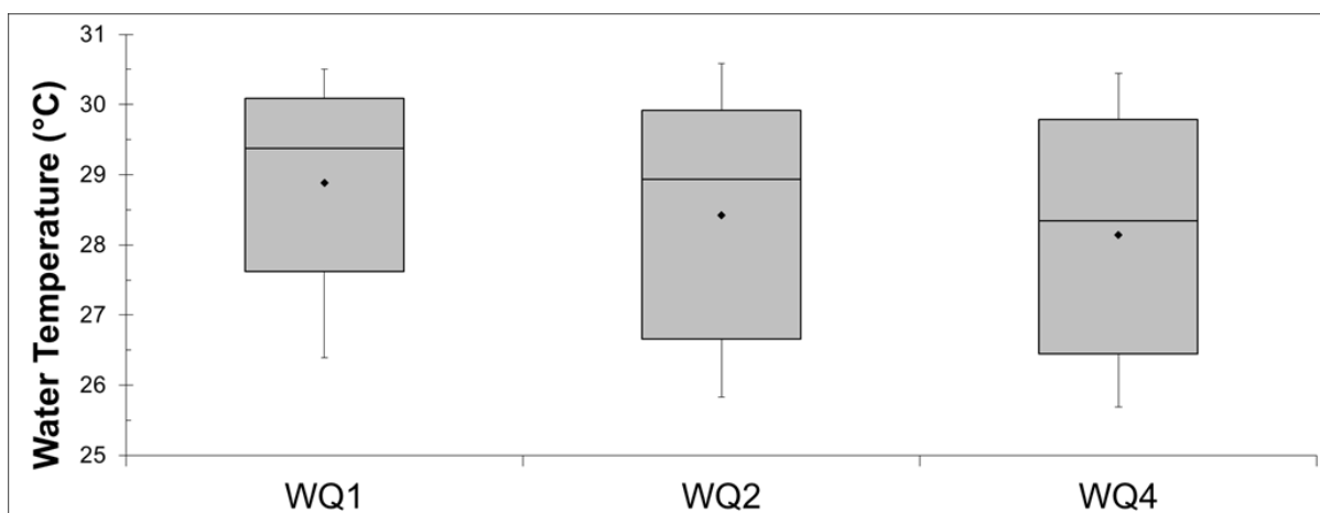
Figure 3.16 Box plot of the water temperature (°C) from July 2020 to July 2021. The lower whisker, lower edge of the box, central line, upper edge of the box and upper whisker represent the 10 th , 25 th , 50 th , 75 th and 90 th percentiles, respectively. The diamond represents the mean value.
