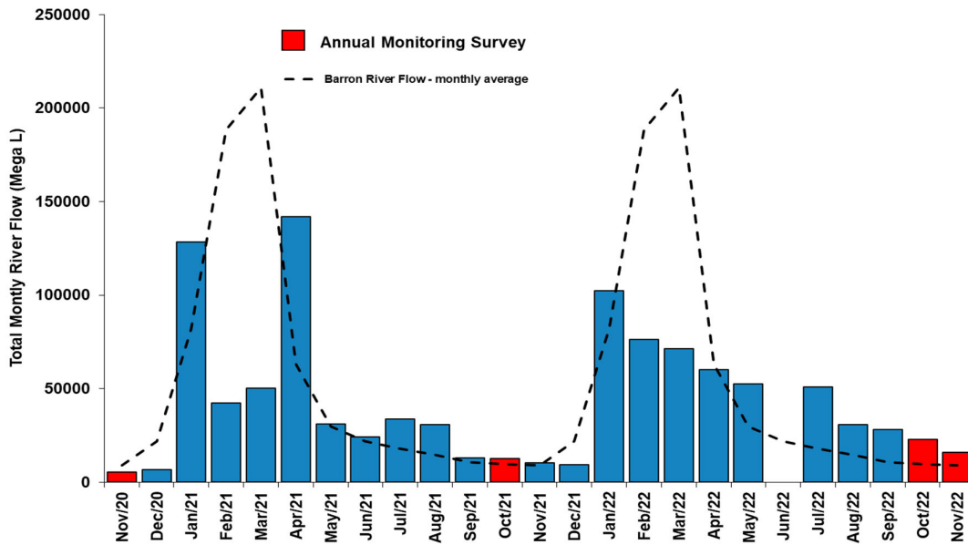
FIGURE 22: MONTHLY WATER FLOW (MEGA LITRES) FOR THE BARRON RIVER RECORDED AT MYOLA, NOVEMBER 2020 TO NOVEMBER 2022. SOURCE: QUEENSLAND DEPARTMENT OF ENVIRONMENT AND RESOURCE MANAGEMENT, STATION 110001D, AVAILABLE AT: HTTP://WATERMONITORING.DERM.QLD.GOV.AU/HOST.HTM
